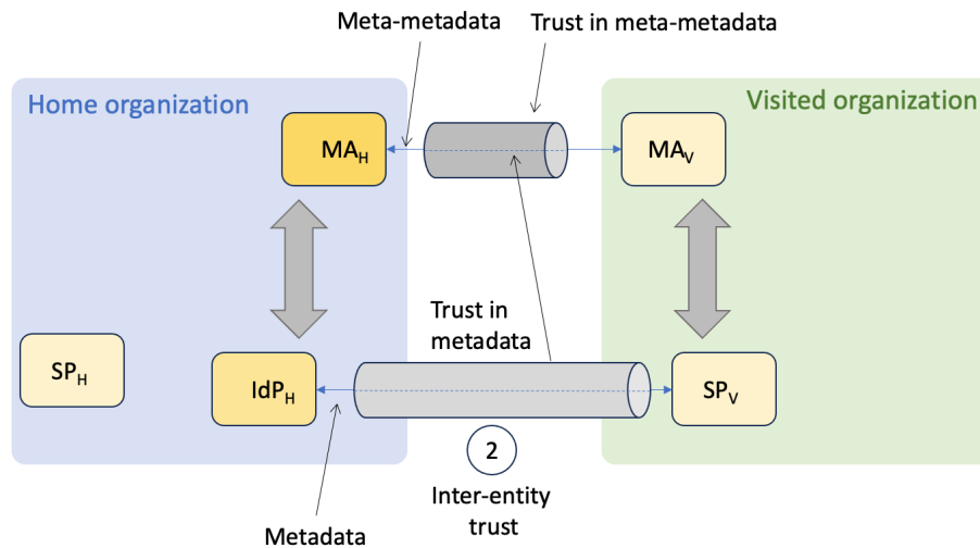
Figure 4: Establishing inter-entity trust between IdP H and SP V
